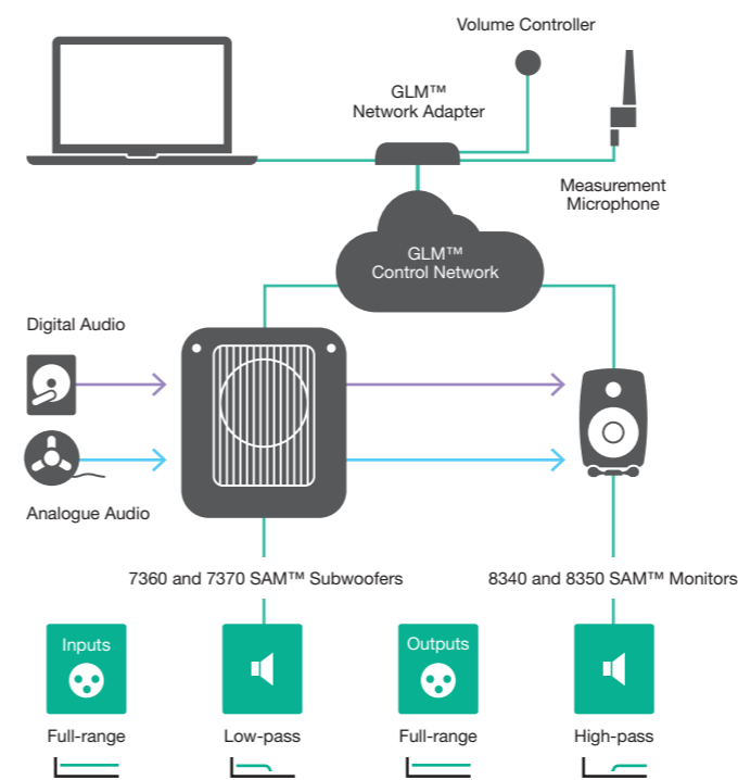
SAM™ System's basic connections and functionalities
