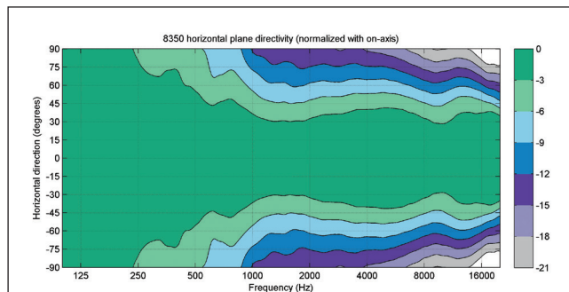
Figure 17. The curves above show the horizontal directivity characteristics of the 8350A.
