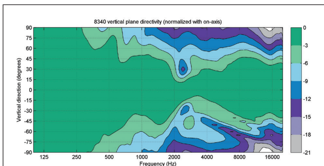
Figure 18. The curves above show the vertical directivity characteristics of the 8340A.
