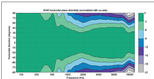
Figure 16. The curves above show the horizontal directivity characteristics of the 8340A.
